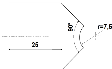
TEMPLATE FOR NOSE-/SPINNER-RADIUS
